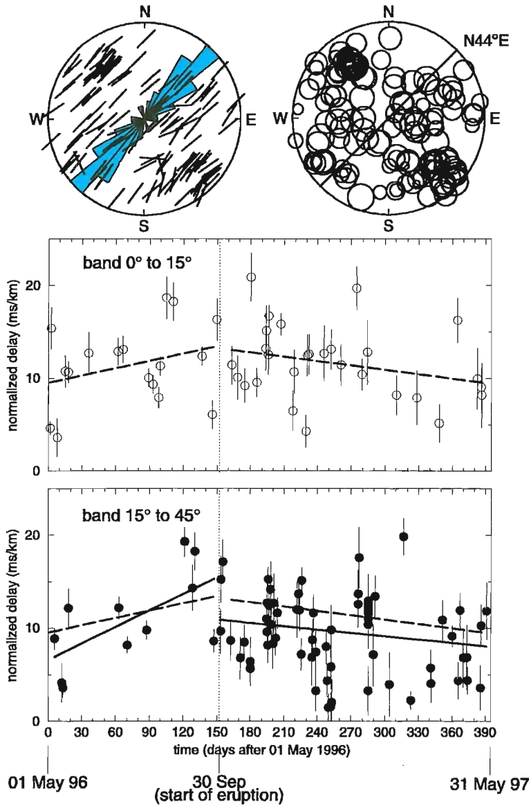
Figure 11: Variations of shear-wave splitting at SAU for 390 days from May 1, 1996. Polar equal-area maps out to 45^\circ of left shear-wave polarizations, with rose diagram indicating average direction, and right circles scaled to normalized time-delays (ms/km). Variation with time of normalized time-delays for ray paths in bands with incidence 0^\circ to 15^\circ to the crack face (sensitive to crack density), and for ray paths in bands with incidence 15^\circ to 45^\circ to the crack face (sensitive to aspect-ratio). Lines are least-squares fits before and after the eruption. Dashed lines in the lower plot repeat lines in the upper plot. Error bars are approximate.
