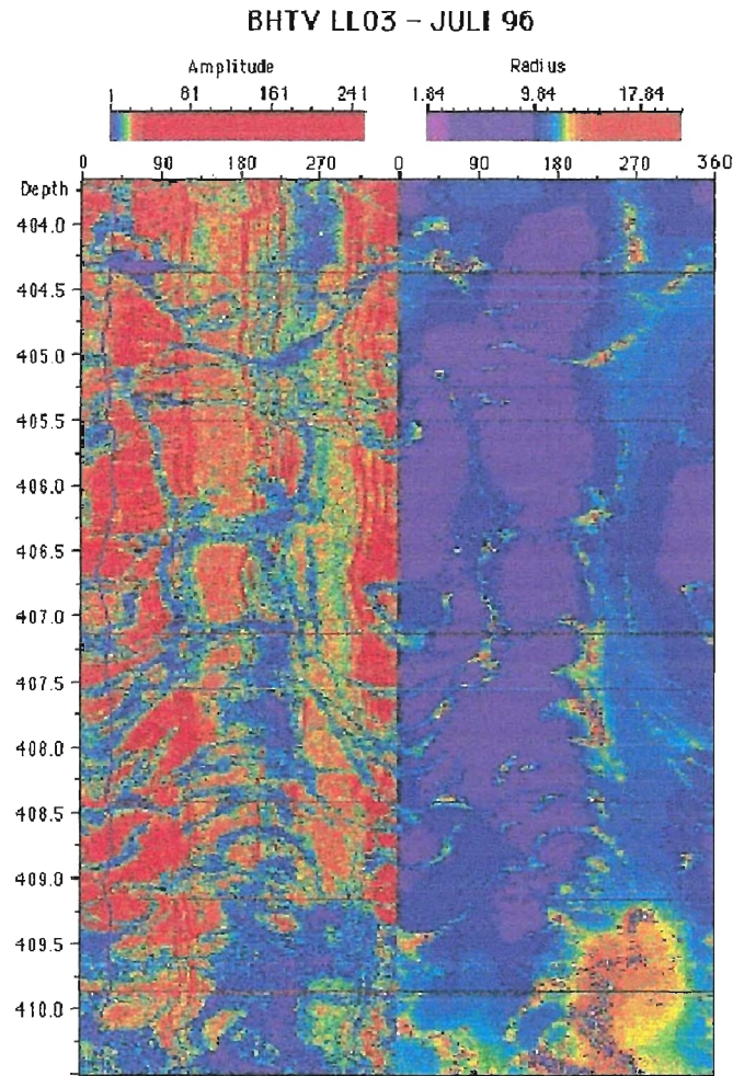
Figure 13: Televiewer logs run in borehole LL-03 in a fractured section. In reading the azimuth scale note that 0 means 320° and 90 means 230°, etc.
