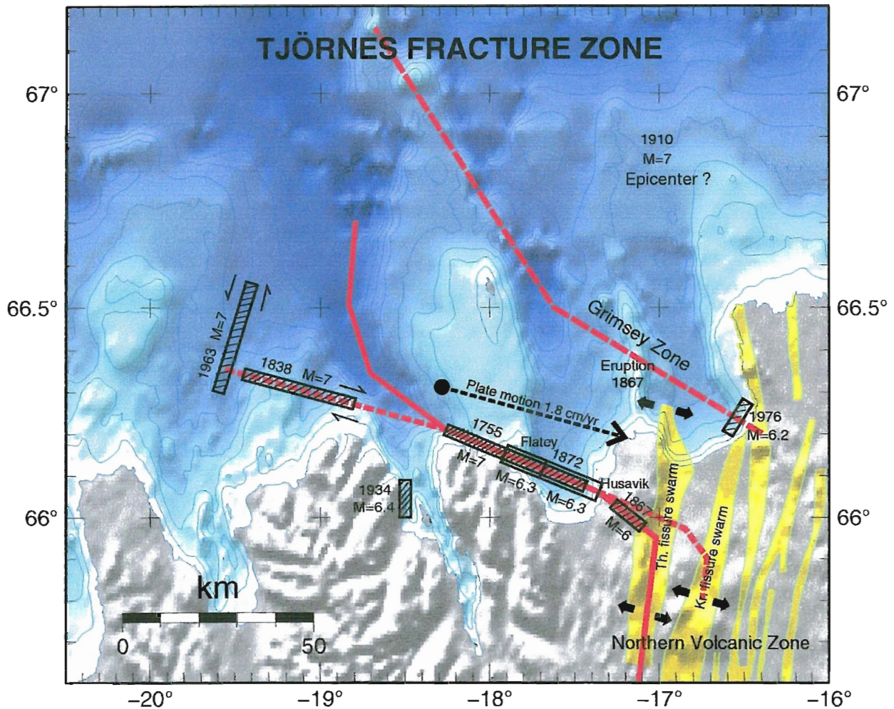
Figure 3: The Tjörnes fracture zone is a complicated right-lateral transform zone which connects the rifting in the northern volcanic zone of Iceland to the ESE-WNW rifting in the Mid-Atlantic rift zone to north of Iceland. The general plate motion according to NUVEL-1A is indicated. The red lines indicate the lines where it is proposed that the most significant transform-rifting motion presently takes place. The most pronounced feature is the Húsavík-Flatey transform fault, which with its proposed westward continuation is the only well developed transform fault of Iceland, up to 10 million years old. Historical seismicity has been interpreted and is assumed to lie mostly on this fault. The Grímsey zone is much more volcanic and geologically a more recent feature. These two zones are proposed to take up the main part of the plate motion. It is not known what is the contribution of each, and it is assumed this is variable with time, depending on changing conditions in and around the fracture zone.
