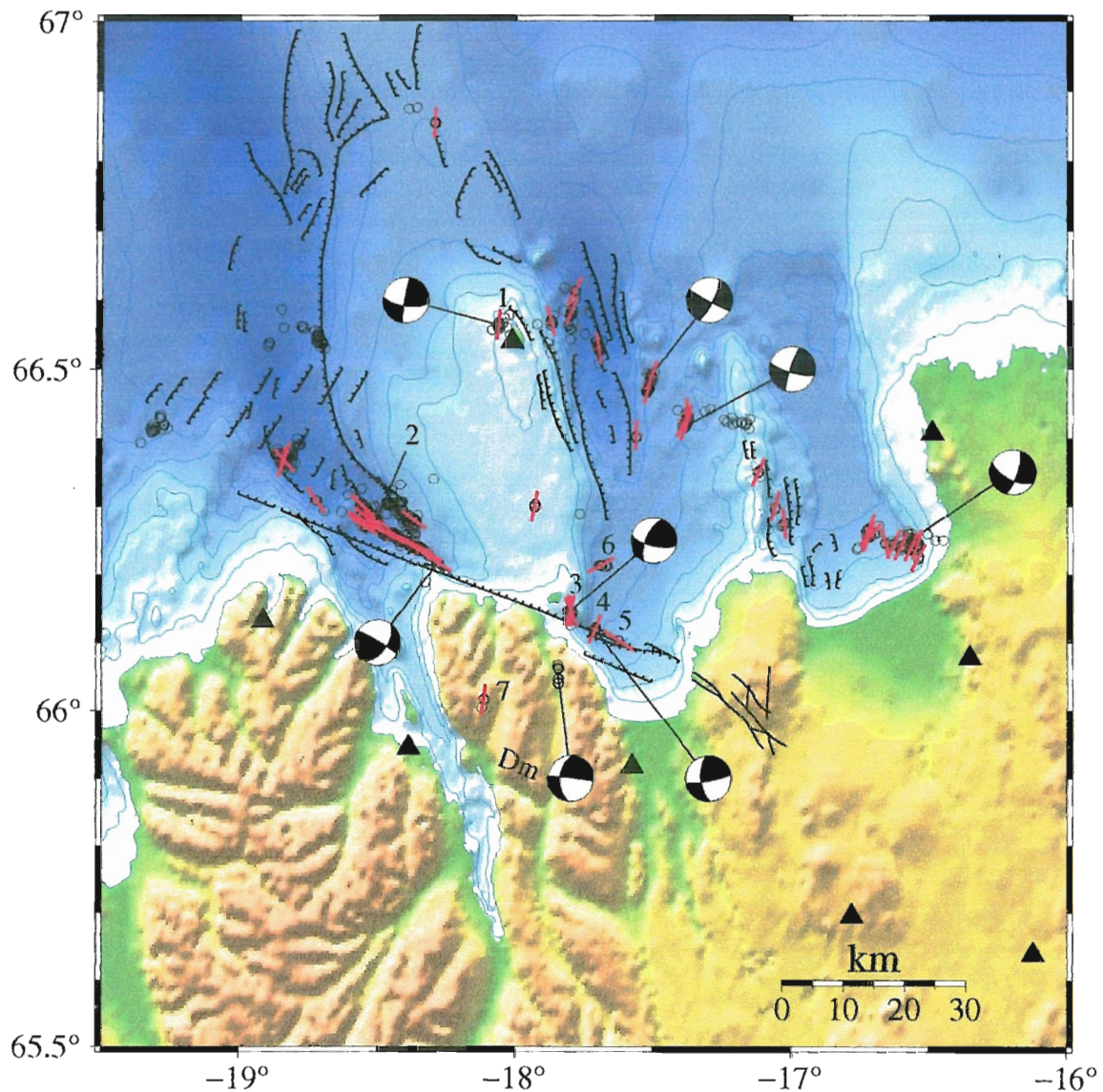
Figure 4: Mapped faults within the Tjörnes fracture zone off the north coast of Iceland. Black lines indicate faults mapped with conventional reflection seismic methods or by direct observations on-land. Red lines are 60 active fault segments mapped using accurate relative locations of microearthquakes recorded by the SIL network. Seismic stations are denoted by triangles. Dark patches are sites of recent volcanism. The depth contour interval is 100 m.
