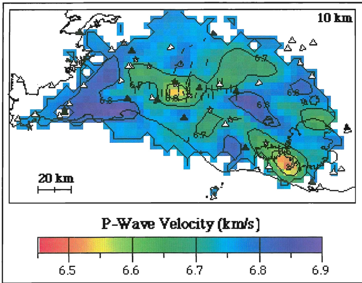
Figure 8: 3-D P-wave velocity at 10 km depth in the crust beneath SW-Iceland estimated from local earthquake tomography.
