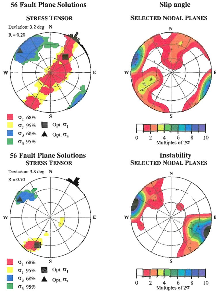
Figure 7: Same 56 microearthquakes as in the previous figure but now inverted with different nodal plane picking algorithms. Both examples in this figure have been inverted with acceptable fault plane solutions (fps). The upper row is the same as the lower row in the previous figure and used a plane selection criterion based solely on the fit of the theoretically calculated shear-stress direction to the direction of observed slip on the plane. Whichever plane had the smallest misfit angle was chosen. In the lower row a more physical criterion was applied. The plane with lowest stability, calculated using a simple Mohr-Coulomb failure criteria, was chosen as the fault plane. This criterion gives a slightly higher average deviation, but as can be seen in the figure, much more well defined principal stress directions. The direction of maximum horizontal compression is likewise more well defined and the stress regime is now more decisively strike-slip. The chosen nodal planes are preferably NE-SW striking subvertical planes for both algorithms although the instability method picks them more frequently and does include very few subhorizontal planes [72].
