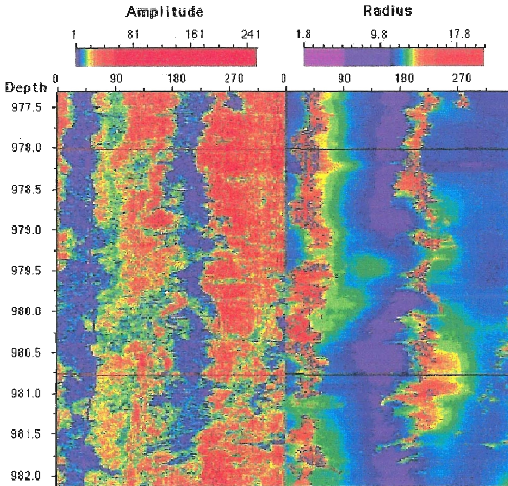
Figure 12: Televviewer logs run in borehole LL-03 in a depth interval containing breakouts. In reading the azimuth scale note that 0 means 320° and 90 means 230°, etc.
