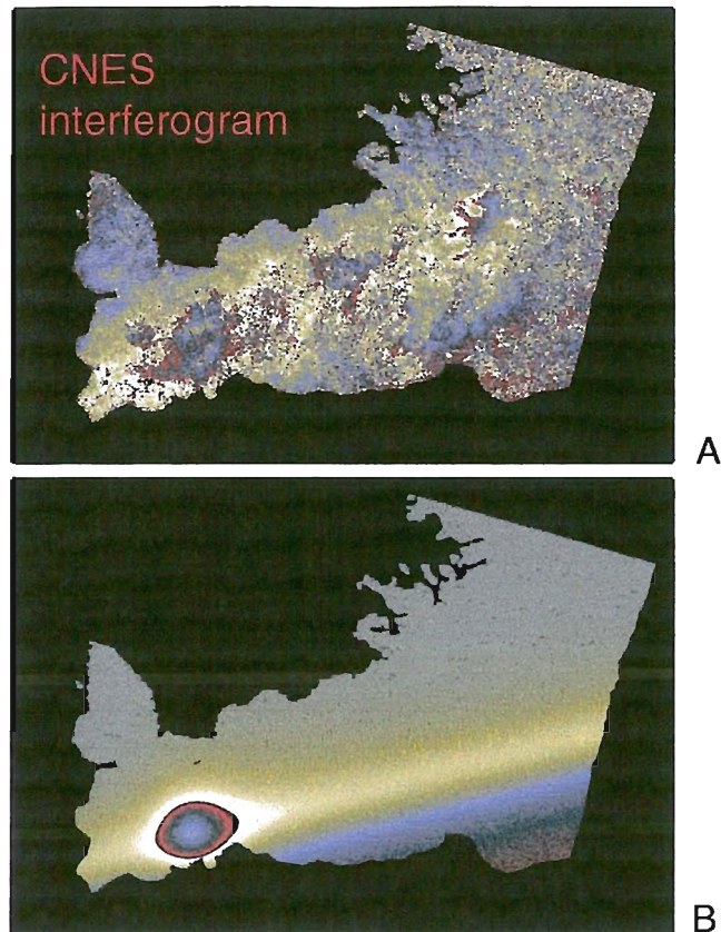
Figure 14: SAR study of the Reykjanes Peninsula, SW-Iceland. Interferogram 2.29 years (A) and model interferogram showing best-fit simulated 2.29-year deformation (B). Time-progressive fringes appearing consistently in the interferograms are indicative of crustal deformation. Phases coded into bytes (8 bits) are represented with a false colour table. A complete colour cycle, for example from blue to blue, represents one complete fringe; a 28-mm change in range in the case of ERS. Concentric fringes are located at the Reykjanes central volcano and manifest a time-progressive increase in range to the satellite. An increase in range along the whole plate boundary, indicative of spreading, is visible as a central fringe in the 2.29-years (A).
