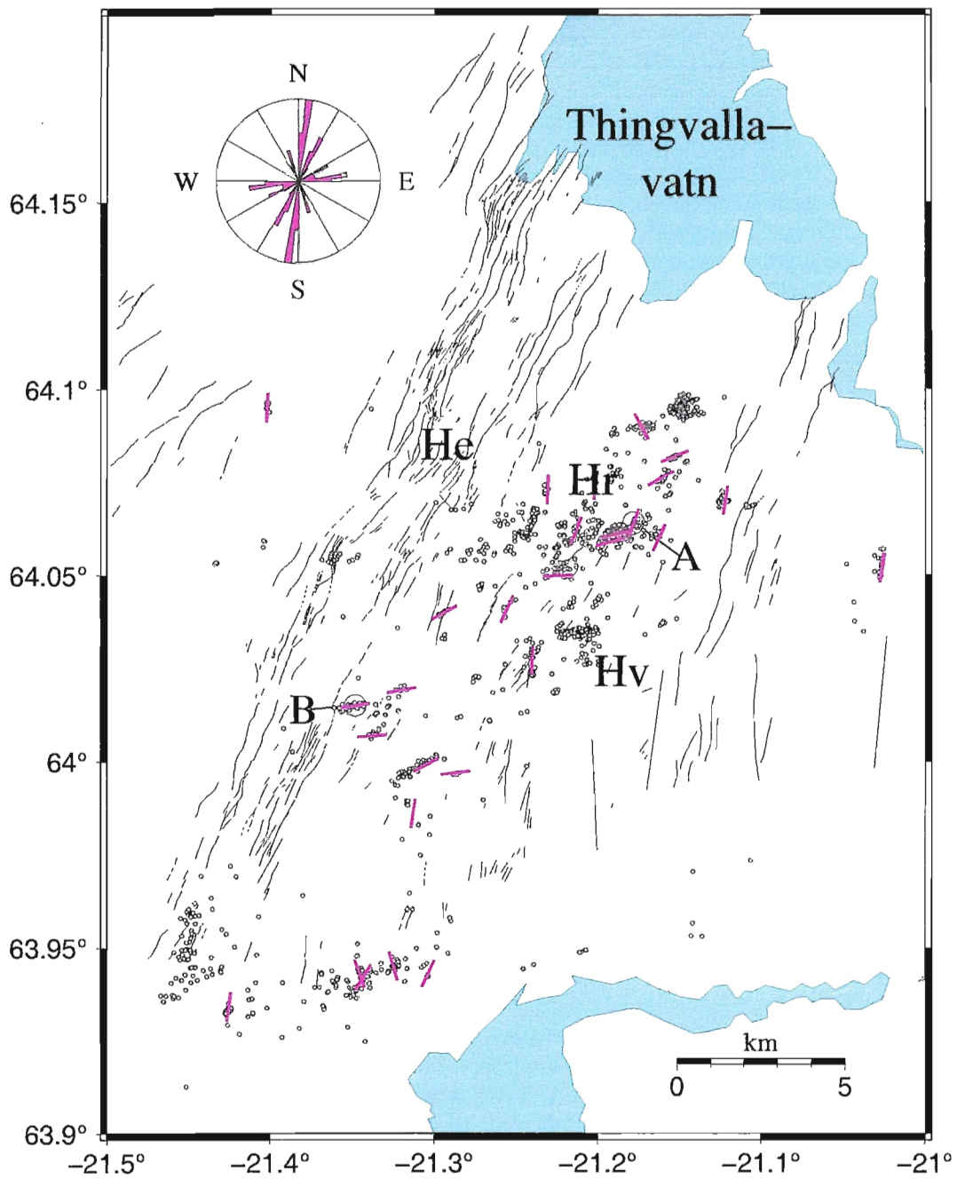
Figure 5: Earthquakes in the Hengill volcanic area, SW-Iceland. The red lines show the location and orientation of fault planes estimated from the relative location of earthquakes. The black lines are mapped surface faults, yellow circles are relocated earthquakes. The inset rose diagram shows the orientation of the 28 faults mapped using accurate relative locations of earthquakes.
