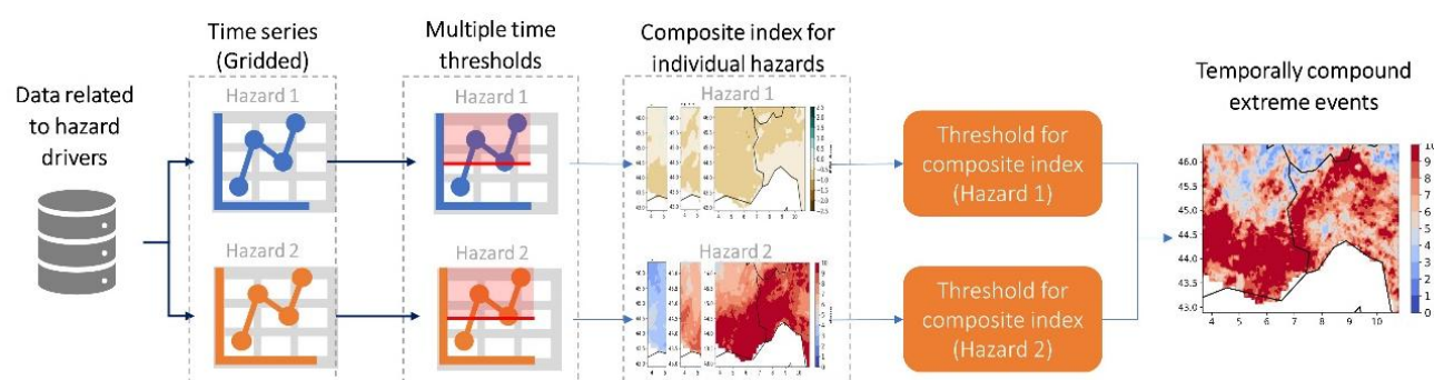
Figure 3.5.1 Framework for estimating frequency of temporally compounding events.
