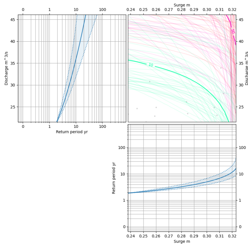
Figure A2.3. Nice compound coastal and riverine flood events at the future (2016-2050) scenario. The figure indicates marginal distribution based on generalized Pareto distribution (GPD) for extreme river flows (upper left), extreme surge (lower right); joint return period of extreme paired data based on the selected copula (upper right).
