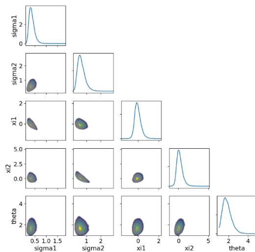
Figure A1.5. Model assessment results for analysing Oslo compound flood events. Corner plots for baseline (a) and future (b) scenarios.
