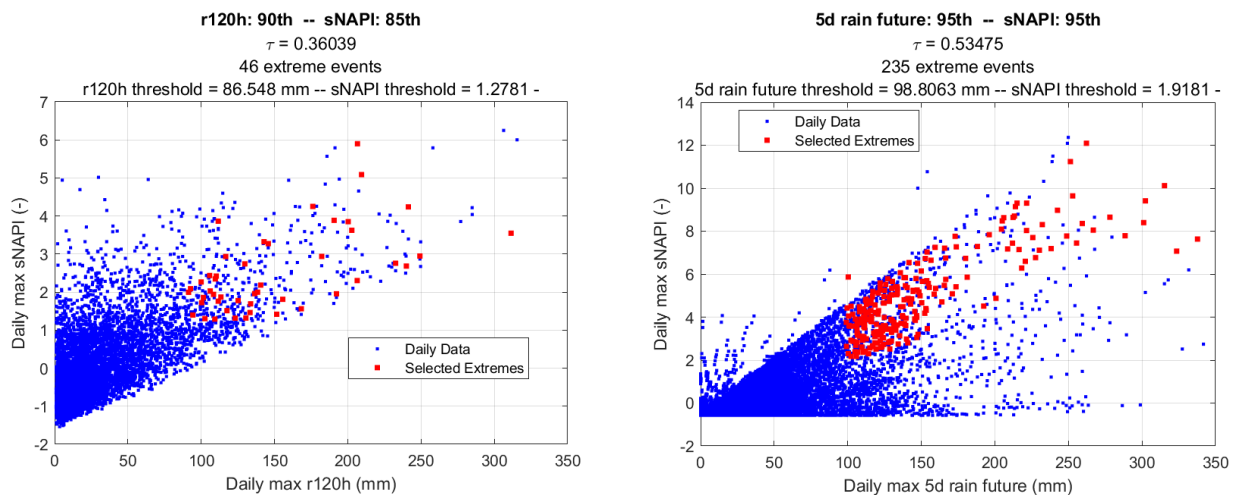
Figure 5.4.2 Joint extreme events. Scatter plot of all pairs of rainfall and sNAPI
