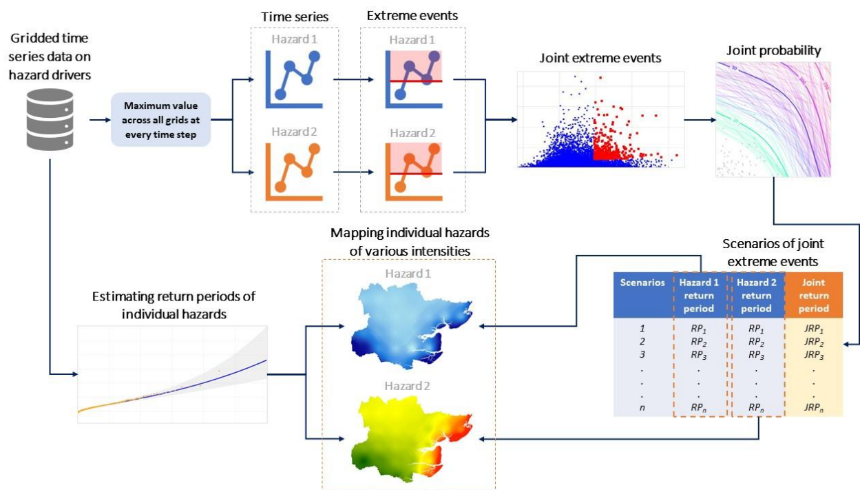
Figure 3.4.1 Framework for analysing spatially compounding events.
