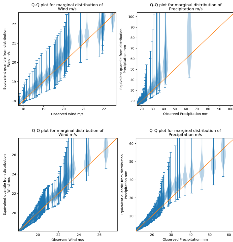
Figure A3.4. Model assessment results for analysing Essex joint extreme wind and rainfall events. Bayesian Quantile-Quantile plots for the two (gust speed and precipitation) marginal GPD, at baseline (upper) and future (lower) scenarios.
