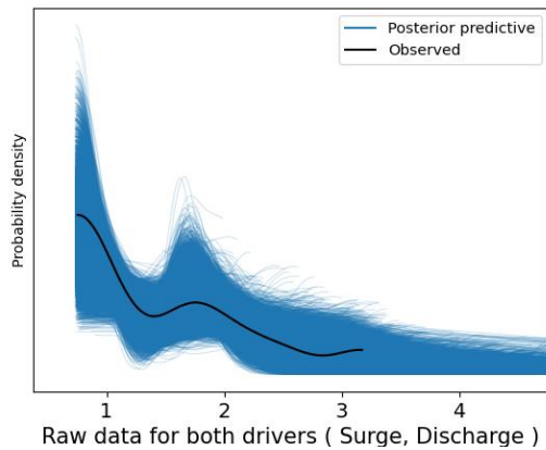
Figure A1.4. Model assessment results for analysing Oslo compound flood events. Posterior predictive checks at baseline (a) and future (b) scenarios
