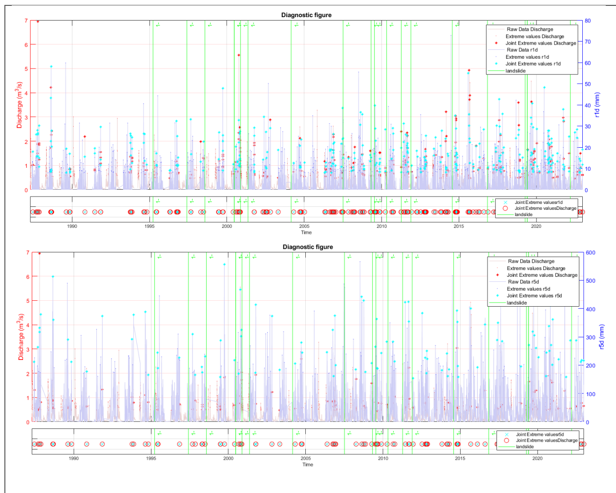
Figure A1.6 Diagnostic figures used to analyse landslide events against joint extreme events. Above 1-day rainfall duration and floods. Below 5-day rainfall duration and floods.
