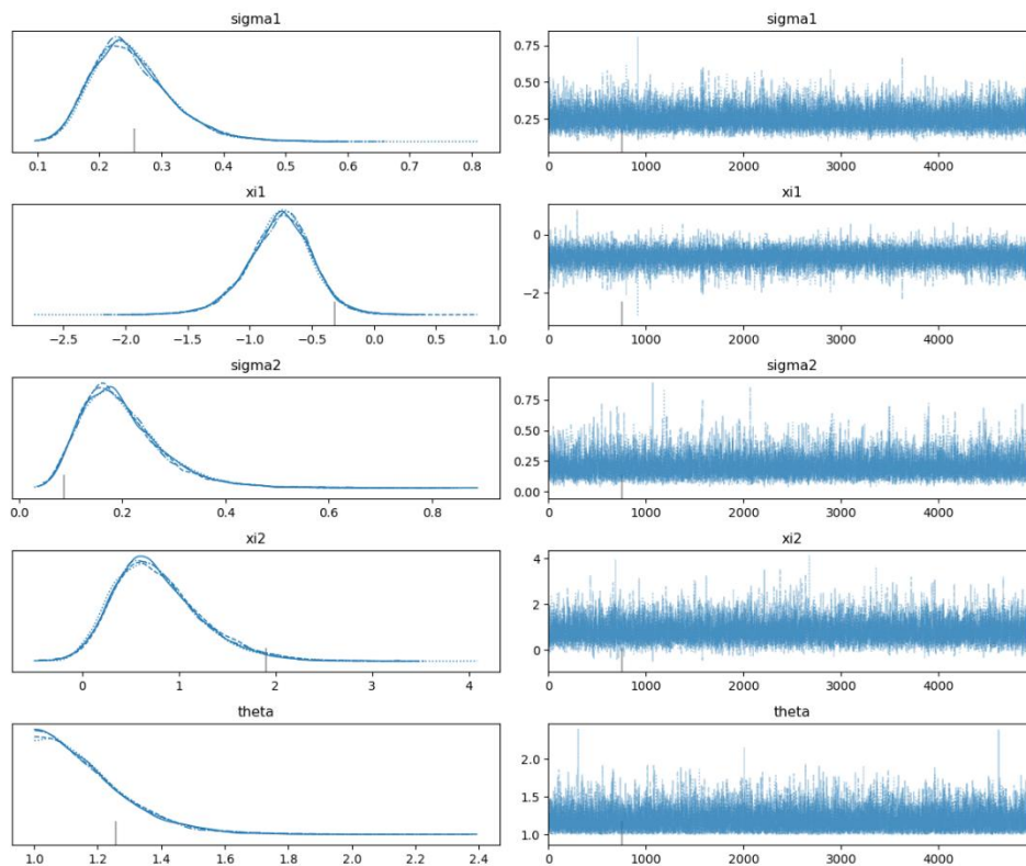
Figure A1.2. Trace plot for the five parameters of the joint distribution function used to analyse compound flood events in Oslo at future scenario. Here, \xi_{i1} and \xi_{i2} are the GPD shape parameters, and \sigma_1 and \sigma_2 are the GPD scale parameters for surge and river flow, respectively. ‘Theta’ is the Gumbel copula parameter.
