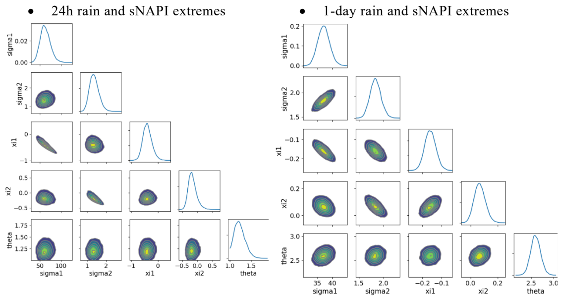
Figure A.4.1 Model assessment results for analysing Múlaping joint extreme rainfall and sNAPI events. Corner plots for historical (a) and future (b) scenarios.
