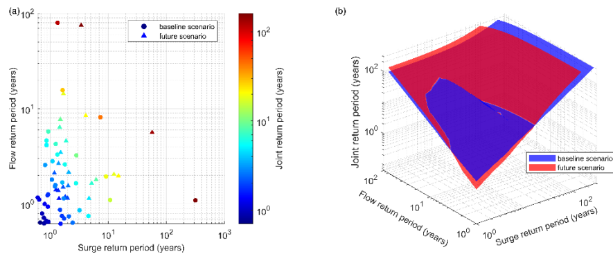
Figure A3.10. Essex compound coastal and riverine flood events. Comparison of JRPs between baseline and future climate change conditions.
