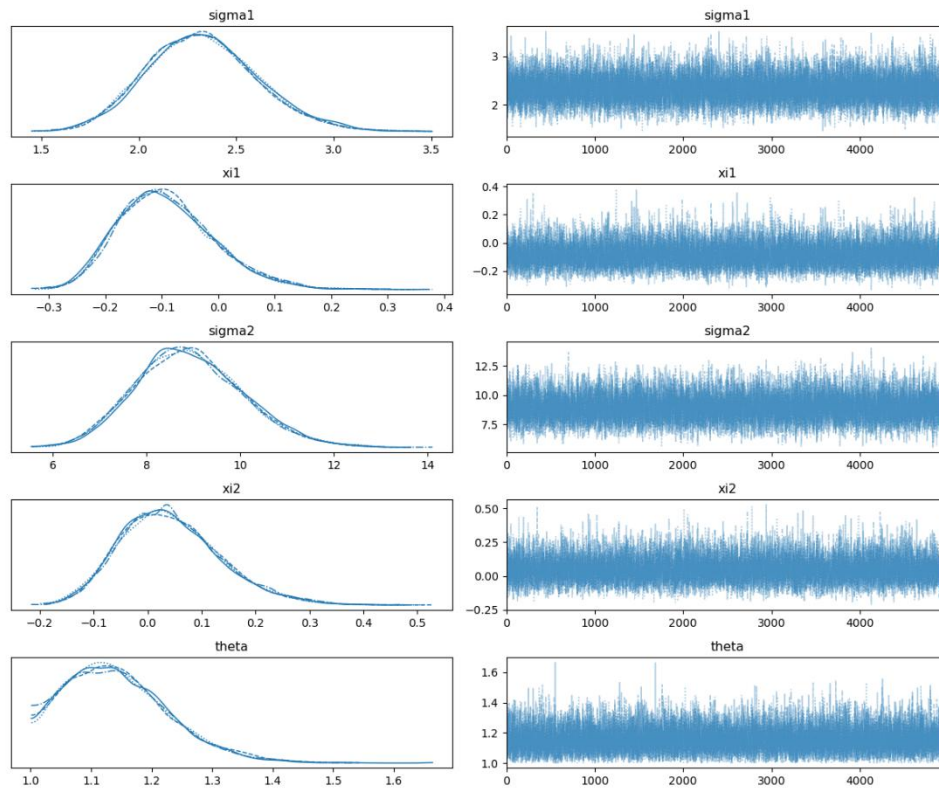
Figure A3.3. Trace plot for the five parameters of the joint distribution function used to analyse joint extreme wind and rainfall in Essex at future scenario. Here, \xi_{i1} and \xi_{i2} are the Generalised Pareto Distribution (GPD) shape parameters, and \sigma_1 and \sigma_2 are the GPD scale parameters for daily maximum wind gust speed and daily precipitation, respectively. ‘Theta’ is the Gumbel copula parameter.
