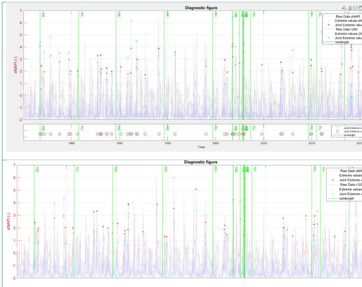
Figure A4.2 Diagnostic figures used to analyse landslide events against joint extreme events. Above 1-day rainfall duration and floods. Below 5-day rainfall duration and floods.
